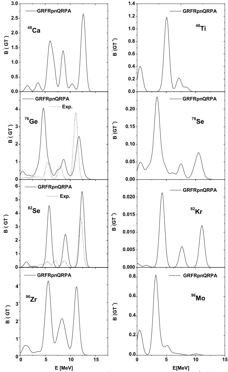
FIG. 3: One third of the single \beta^- (left column) and one third of the \beta^+ (right column) strengths, denoted by B'(GT^-) and B'(GT^+) , for the mother , ^{48}\text{Ca} , ^{76}\text{Ge} , ^{82}\text{Se} and ^{96}\text{Zr} , and daughter, ^{48}\text{Ti} , ^{76}\text{De} , ^{82}\text{Kr} and ^{96}\text{Mo} , nuclei respectively, folded by a Gaussian function with a width of 1 MeV, are plotted as functions of the corresponding energies yielded by the present formalism. Note that the difference of the two strengths for the mother nucleus should amount N-Z if the sum rule is obeyed. For ^{76}\text{Ge} and ^{82}\text{Se} , the experimental data for the \beta^- strength are also presented.
