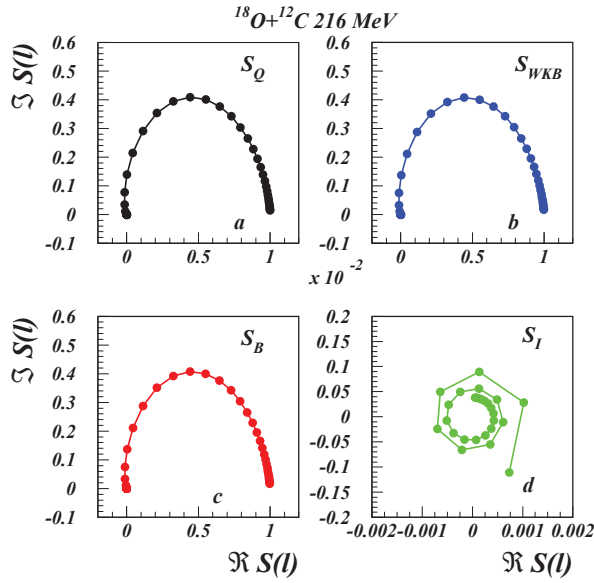
FIGURE 13. (Color online) Argand diagram for the semiclassical S-matrix based on the WS potential equivalent to JLM1. The barrier trajectory (panel b) is identical to the exact quantum result (panel a). The small internal barrier component (panel d) shows a hint of an orbiting effect or the presence of Regge poles, but these are too far from the real axis to have noticeable effect in the total cross section.
