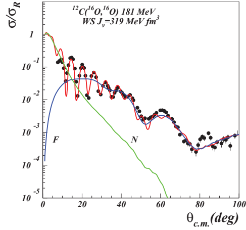
FIGURE 4. (Color online) Elastic scattering {}^{16}\text{O}+{}^{12}\text{C} at 11.3 MeV/nucleon. The real part of the WS optical potential is much stronger and the far side component shows several deep Airy oscillations. Experimental data are taken from [12].
