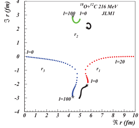
FIGURE 10. (Color online) Complex turning points for the WS potential equivalent to JLM1. The stars denote the complex poles of the potential.
