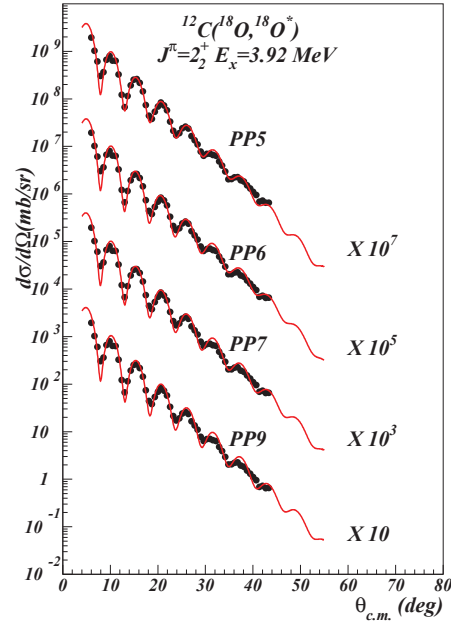
FIGURE 16. (Color online) Inelastic cross section to 2_2^+ (3.92 MeV) state in ^{18}\text{O} . The DWBA calculation is based on the potentials in Table 1.
